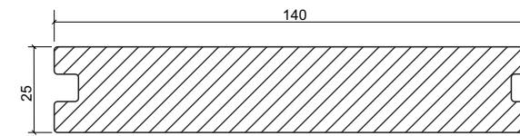
140x25mmx5.4m
