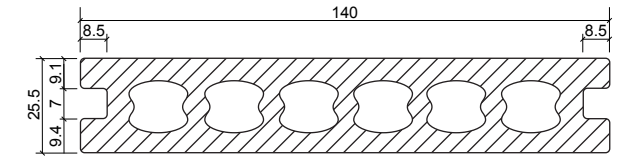
140x25mmx5.4m
